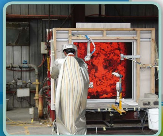
Bush fire testing in process
